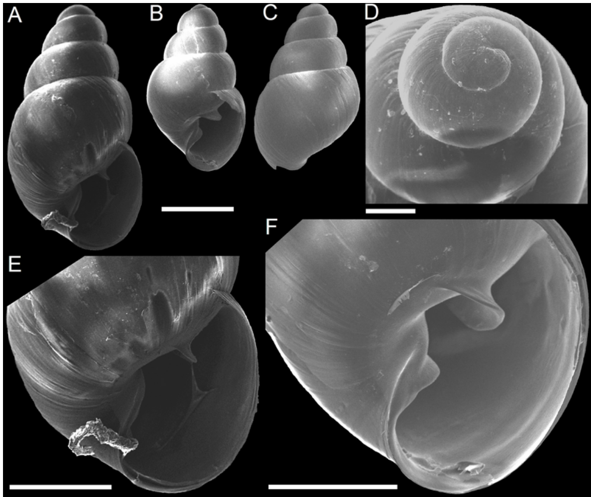
Figure 1. SEM images of Pacificella variabilis Odhner, 1922. A) adult shell, apertural view; B) juvenile shell, apertural view; C) juvenile shell, abapertural view; D) detail of protoconch of juvenile specimen; E) detail of aperture of adult specimen; F) detail of aperture of juvenile specimen.
