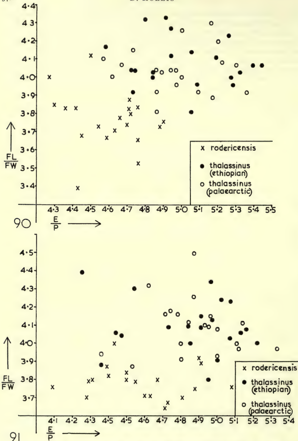
FIGS. 90-91. A. thalassinus ssp., scatter diagrams comparing values of FL/FW against E/P. 90, males; 91, females.
